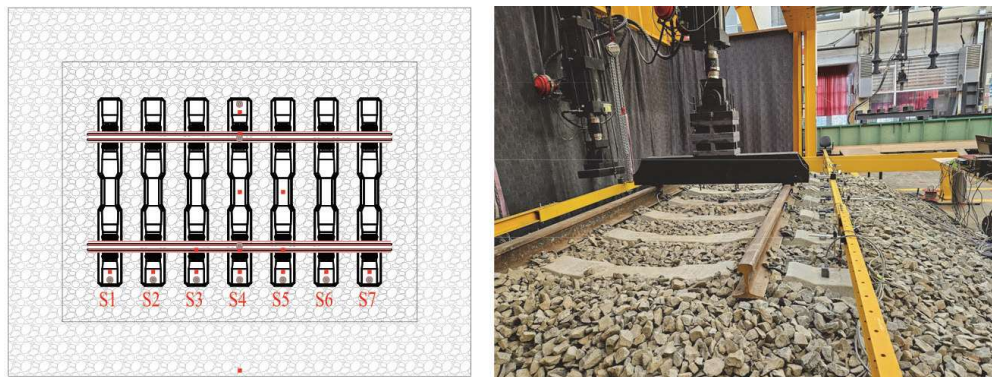
Figure 4 Instrumented track
