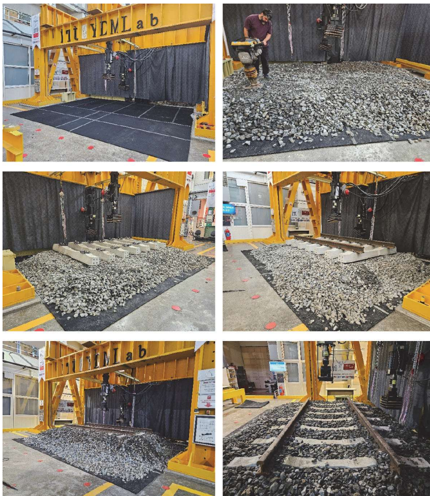
Figure 2 Installation of ballasted track
