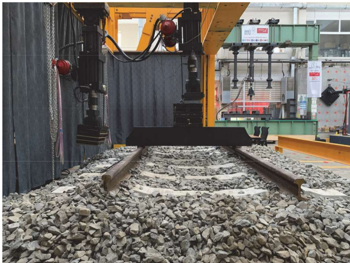
Figure 3 Load distribution beam
