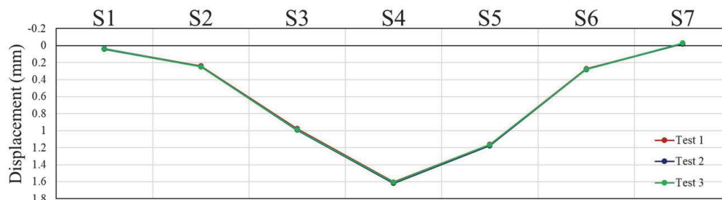
Figure 5 Displacement curve
